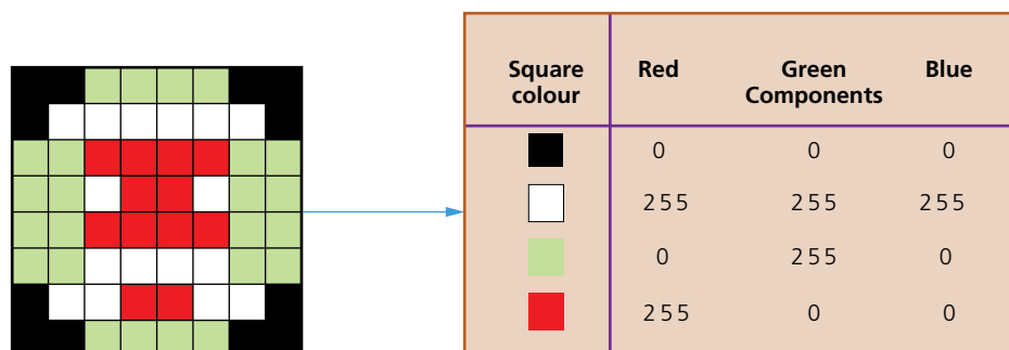
▲ Figure 1.8 Using RLE with a coloured image
